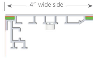
The Silicone strip (green) gets stitched to the graphic perimeter (red) and inserted into the channel for a drum tight fit.
